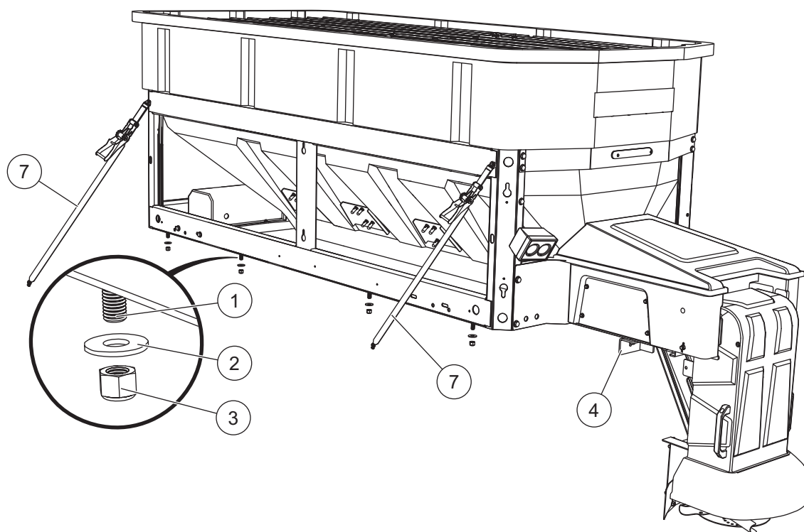
Rear Stop Bracket Fasteners
