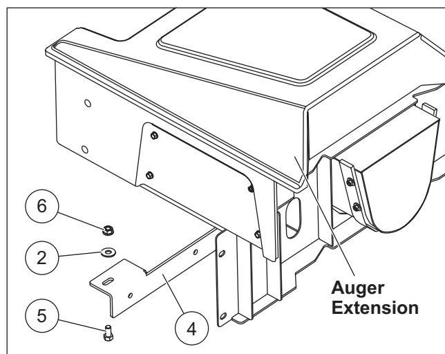
Rear Stop Bracket Fasteners
